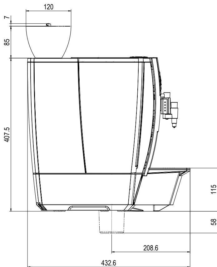
Side outline
