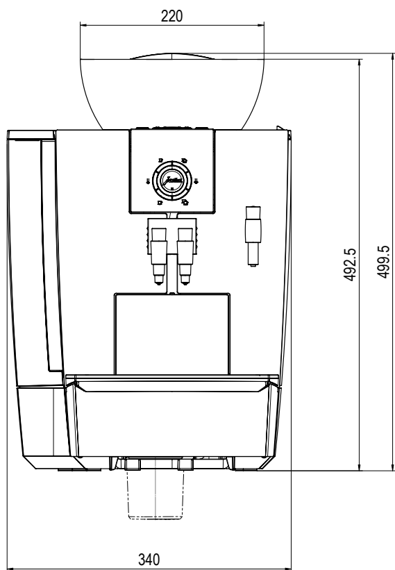
Outline
