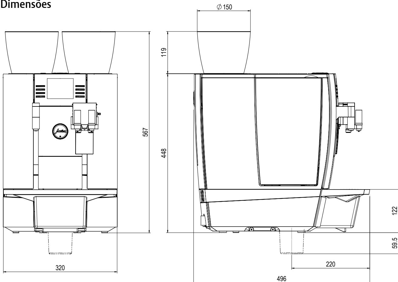
Vista frontal
